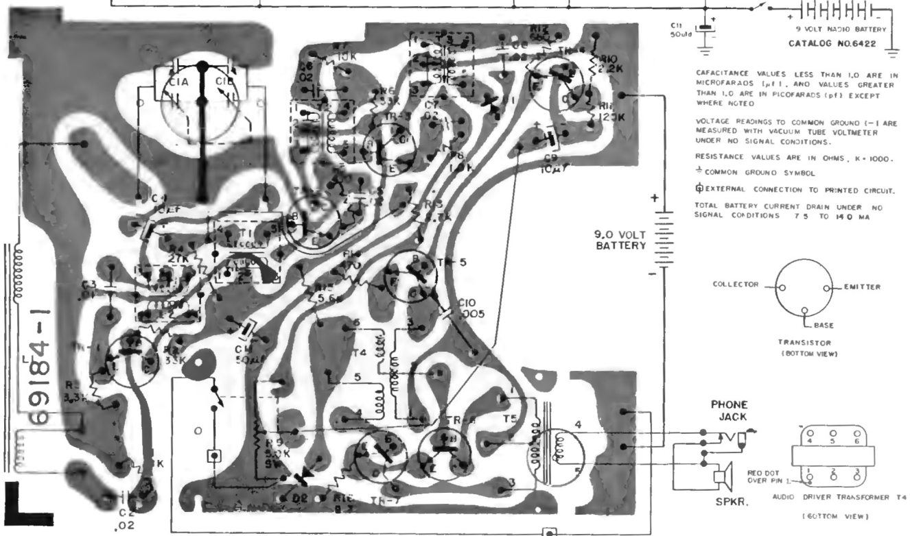
CIRCUIT BOARD DIAGRAM (Bottom View)
