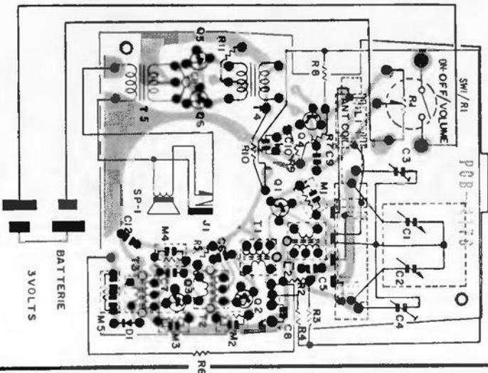
Wiring Side of Printed Circuit Board
