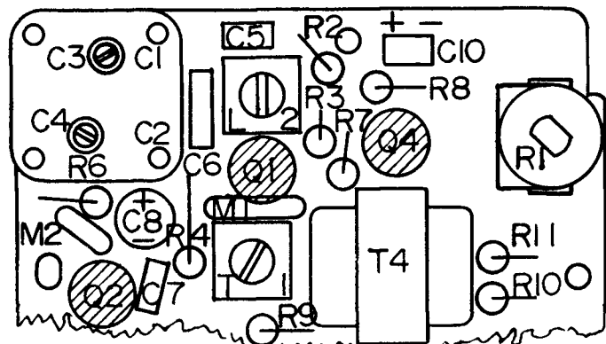
COMPONENT SIDE OF PRINTED CIRCUIT BOARD
