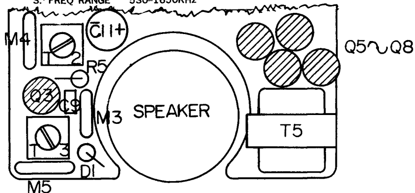
COMPONENT SIDE OF PRINTED CIRCUIT BOARD
