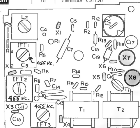
Mounting Diagram
