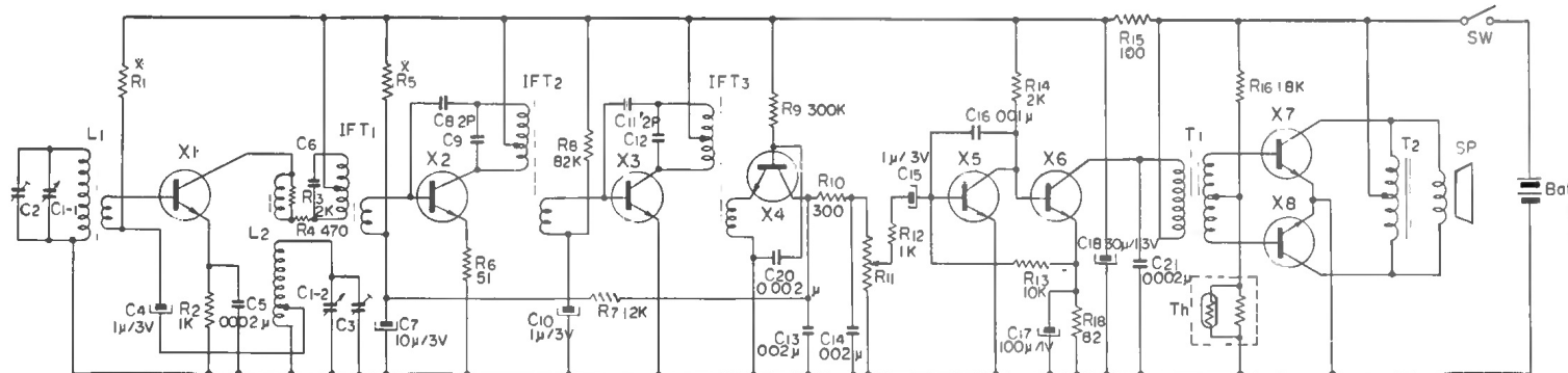
Schematic Diagram
