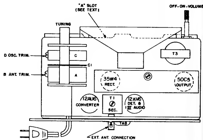
FIG 2 Chassis Layout
