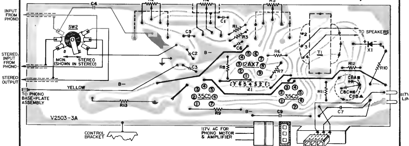
Bottom view of PC board showing top components as schematic symbols.
