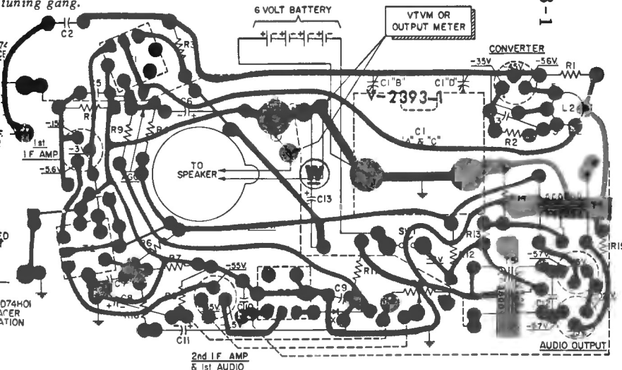
BOTTOM VIEW OF PRINTED CIRCUIT CHASSIS SHOWING COMPONENTS SYMBOLICALLY
