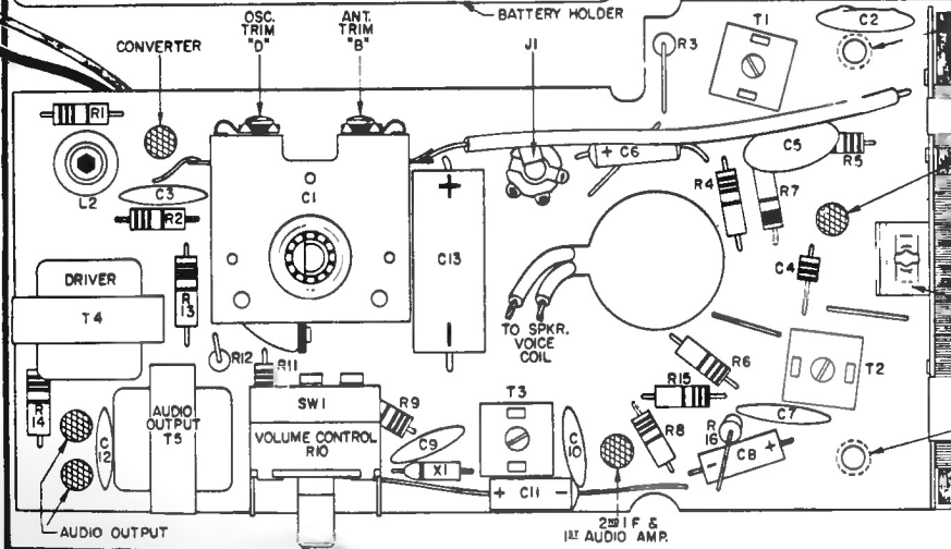
TOP VIEW OF PRINTED CIRCUIT CHASSIS
