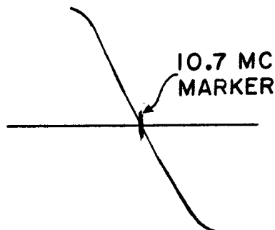
Figure 6 - Discriminator response curve
