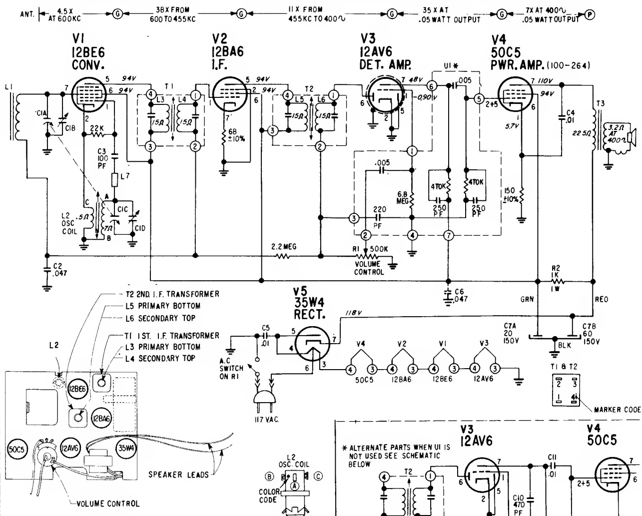
TUBE & TRIMMER LAYOUT CHASSIS 5M04
