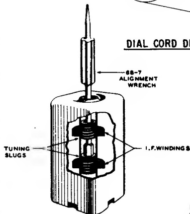
Detail of IF Transformer
