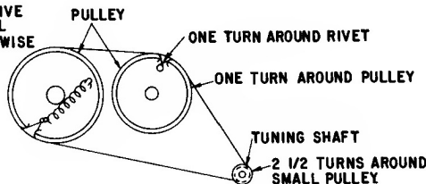
DIAL CORD DRIVE
