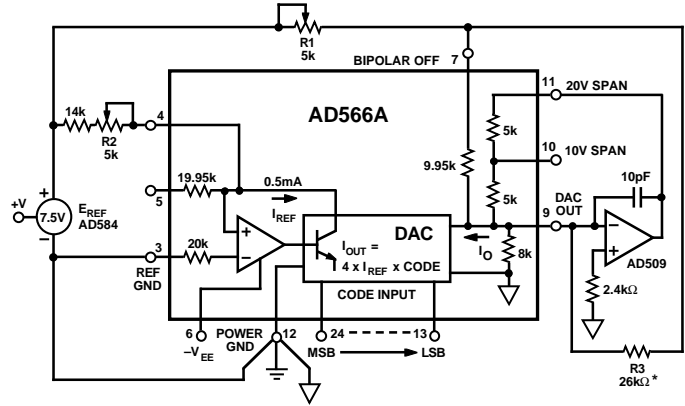
Figure 6. ±10 V Voltage Output
